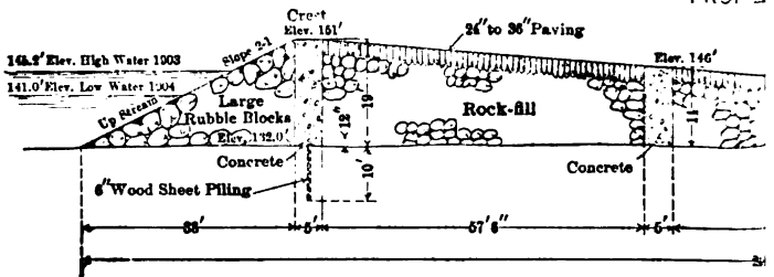
FIG. 180.—Plan and Section
